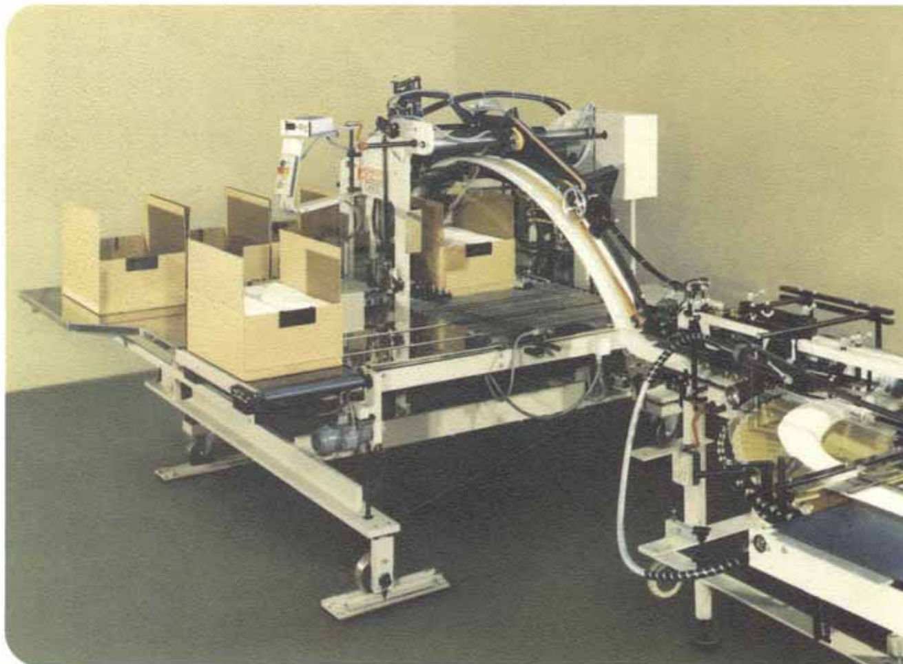
JAPACK 40-2 Universal Folding Carton Packer.
